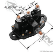
Motor Reversing Solenoid 12V 577.3062
